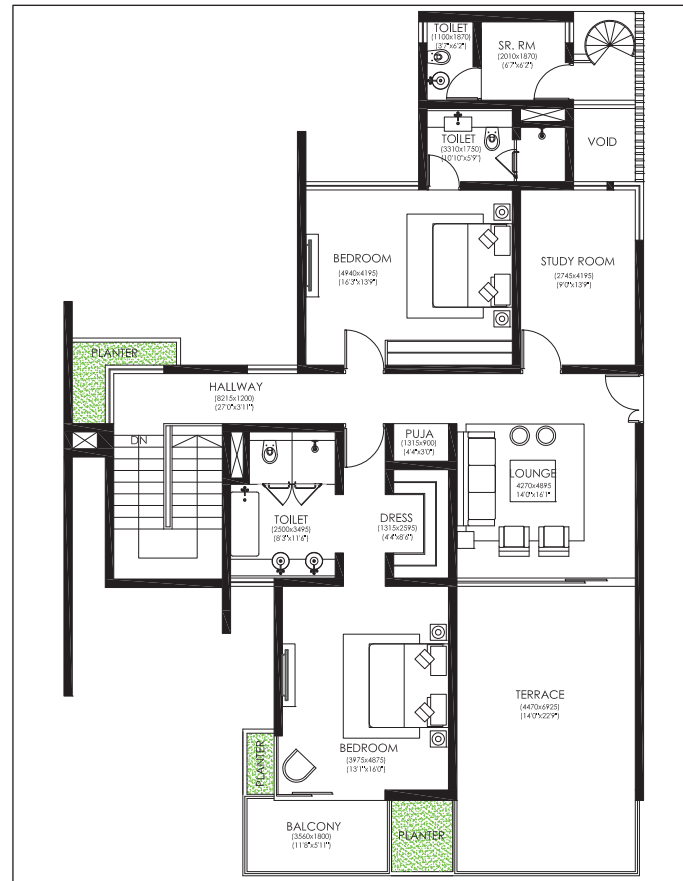
UPPER LEVEL FLOOR PLAN OF DUPLEX IN MID-RISE
